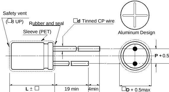
RADIAL LEAD TYPE (立式)
