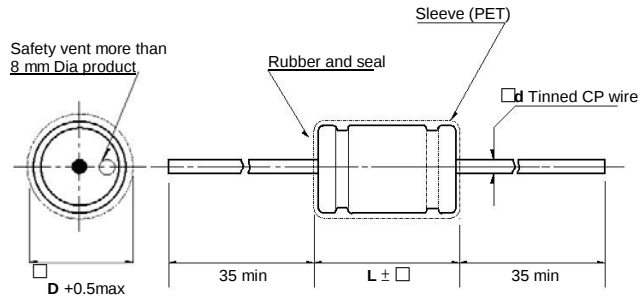
AXIAL LEAD TYPE (臥式)
